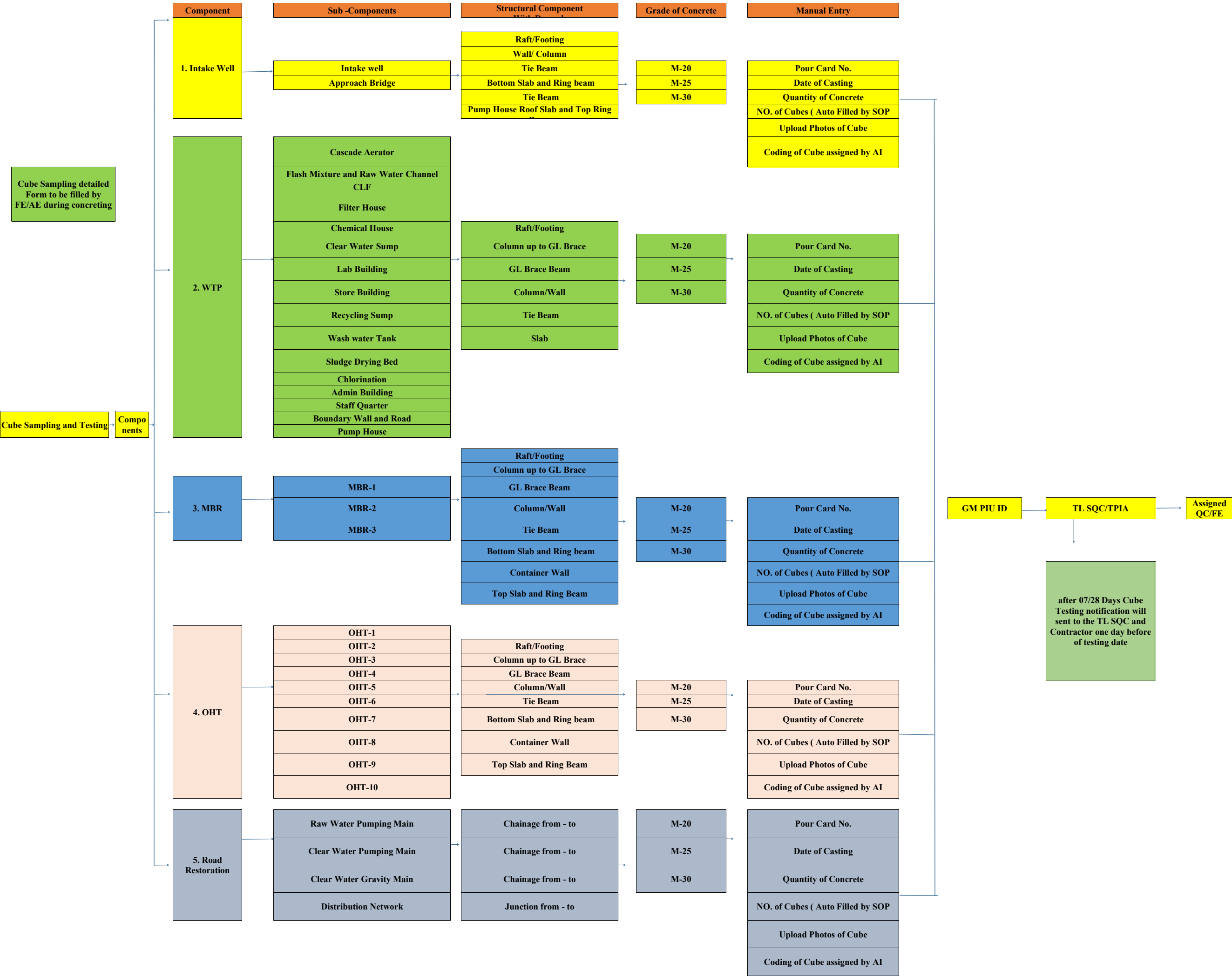
Flow Chart for Cube Testing
